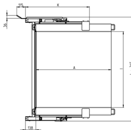
PUA579-CS/FL/FM dimensions with lifting system
